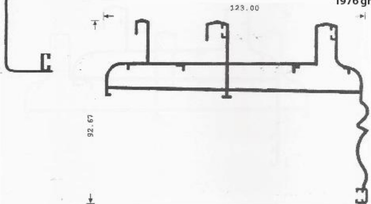
Triple track frame with dicorative cover V 170-06
