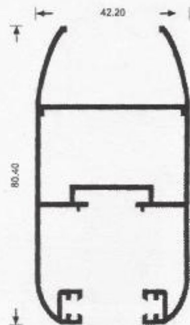
NEW V 170-08/A Anti mosquito leaf frame 5913 gr/m
