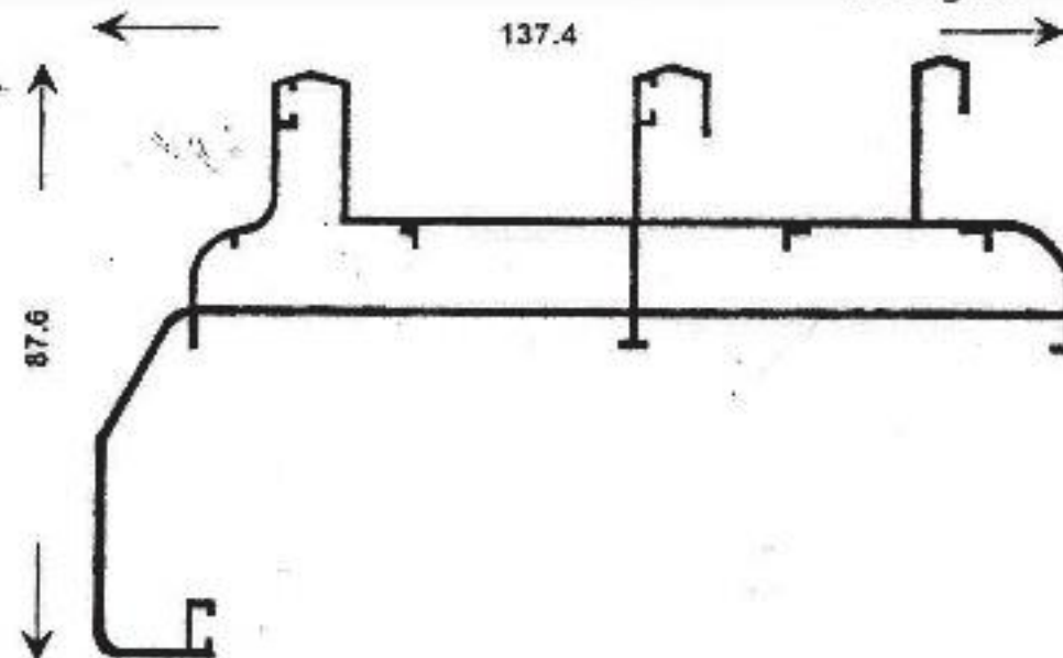
Outer frame with anti - mosquito barrier Inox V 170-06/A
