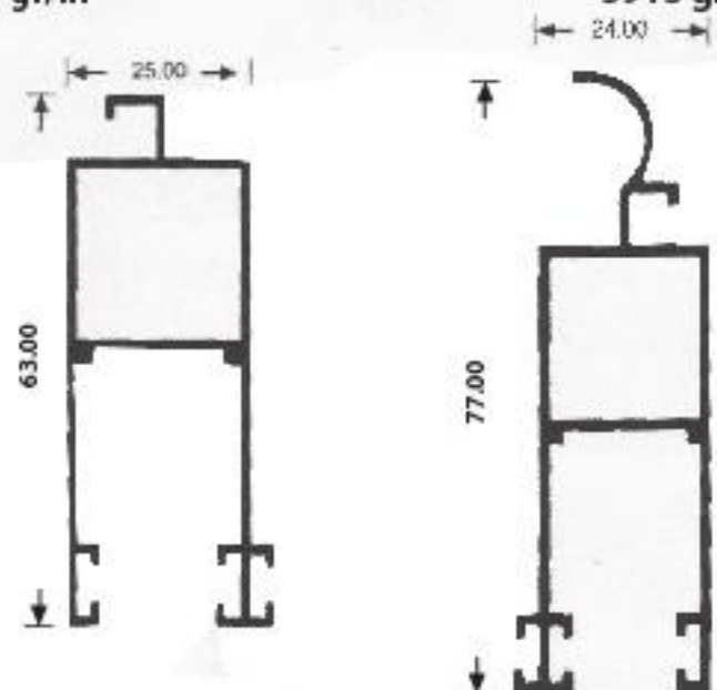
V 170-08 Anti mosquito leaf frame 690 gr/m
