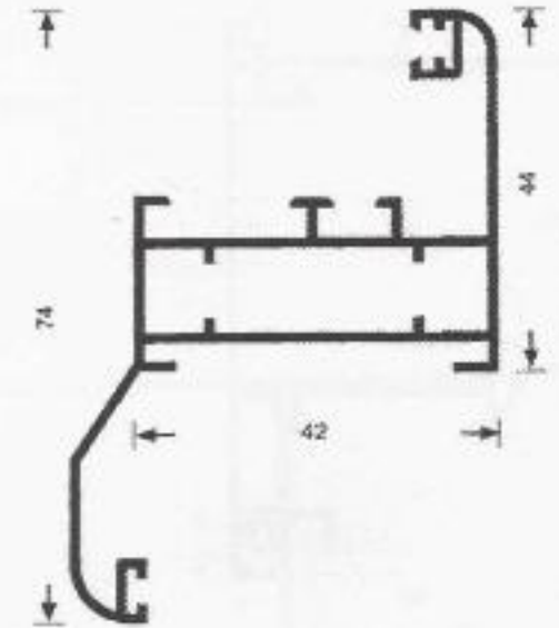
Sash for double glazing small
