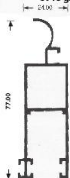
V 170-08 Anti mosquito leaf frame 690 gr/m
