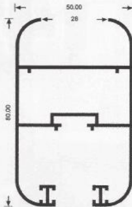
Double glass leaf V 140-04 1246 gr/m
