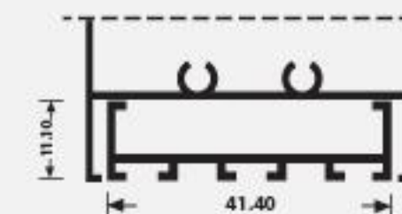
Bottom frame anti- moisture profile V 120-20 375 gr/m
