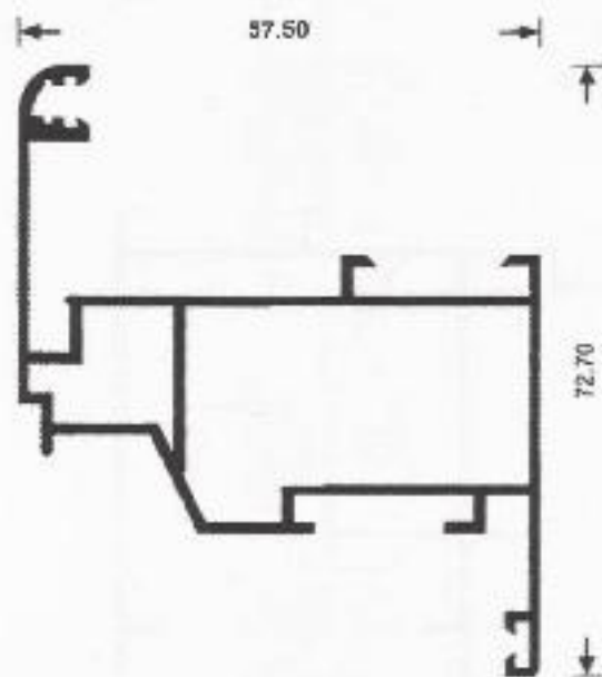
Small leaf frame V 120-02 1167 gr/m
