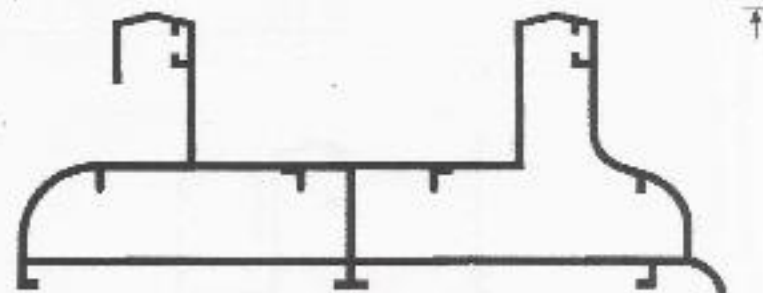
Double track frame with anguler cover V 170-10/A
