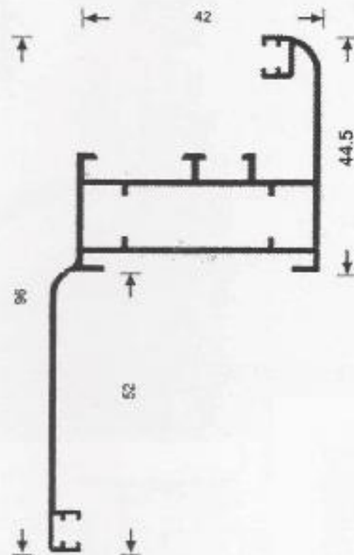
MV 204/B W = 972 gr/m
