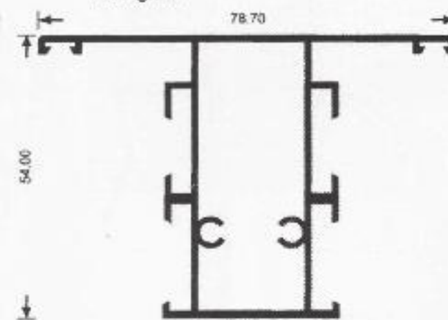
Cover V 120-12A 917 gr/m
