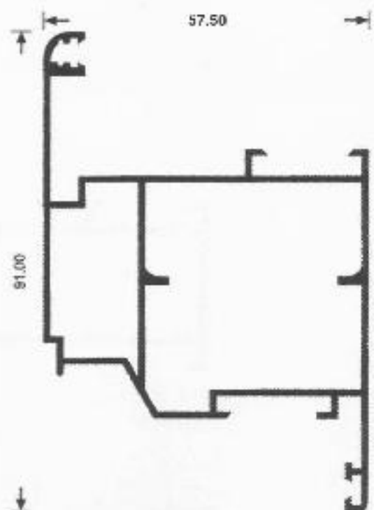
Medlum leaf frame V 120-03 1334 gr/m
