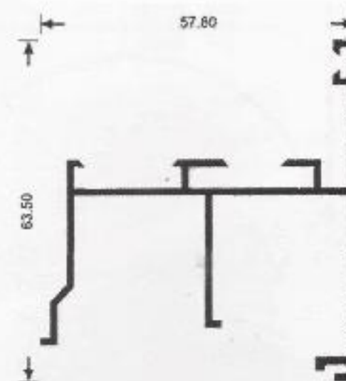
Bottom frame anti- moisture profile V 120-20 375 gr/m
