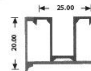
Fillet for a single window V 170-05/A 270 gr/m
