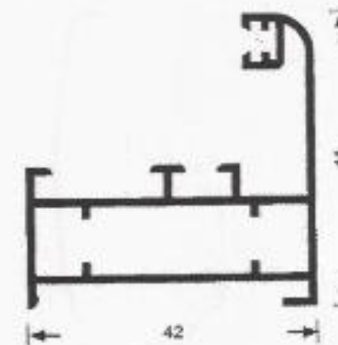
MV 205/A W = 694 gr/m
