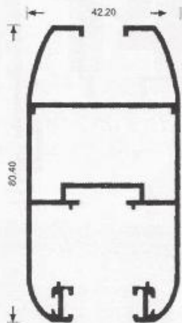
Single glass leaf frame V 170-07 1250 gr/m
