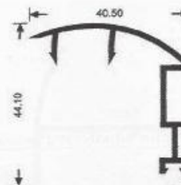
Multiple holding bracket V 170-03 400 gr/m
