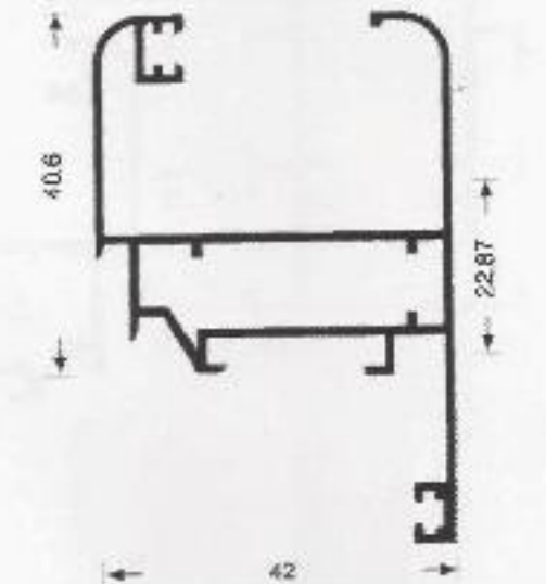
MV 207/A W = 800 gr/m
