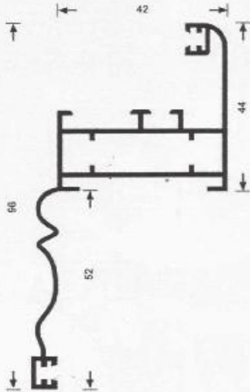
MV 204/A W = 972 gr/m
