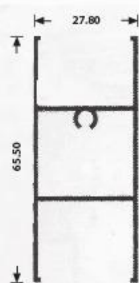
NEW V 170-08/A Anti mosquito leaf frame 5913 gr/m
