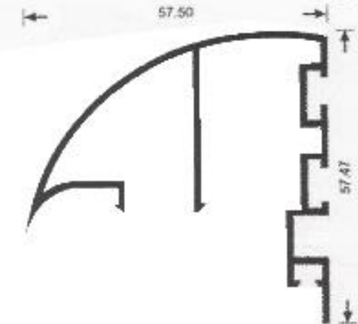
Decorative cover V 140-07 330 gr/m
