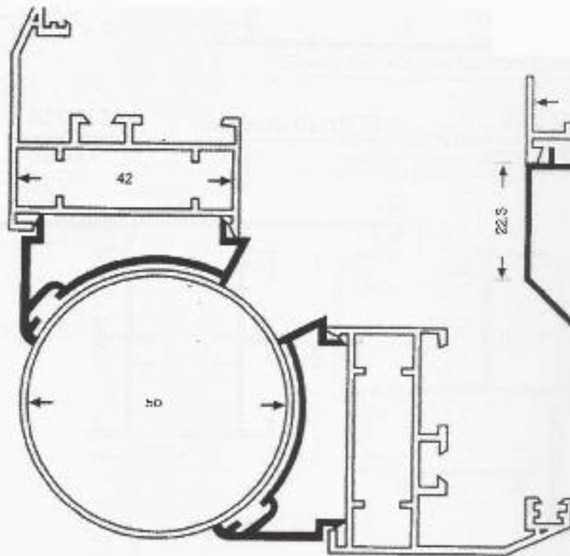
Profile for adjustable corner column MV 221 W = 317 gr/m
