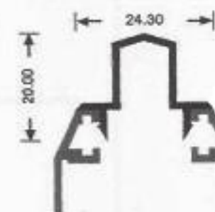
Hidden fillet for leaf frame V 170-04/A 250 gr/m
